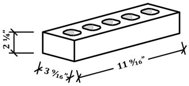
SUMMIT PLANT NORMAN
