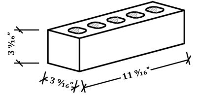
SUMMIT PLANT UTILITY NORMAN (4x4x12)
