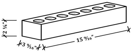
SUMMIT PLANT SUPER SIXTEEN INCH NORMAN
