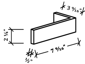
SUMMIT PLANT THIN BRICK CORNER
