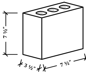
SUMMIT PLANT TRIPLE BRICK
