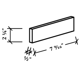
SUMMIT PLANT THIN BRICK
