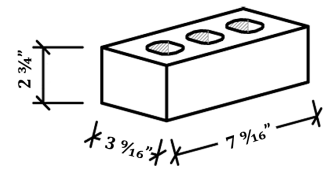
SUMMIT PLANT ENGINEER MODULAR
