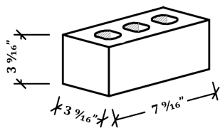
SUMMIT PLANT CLOSURE (4x4x8)
