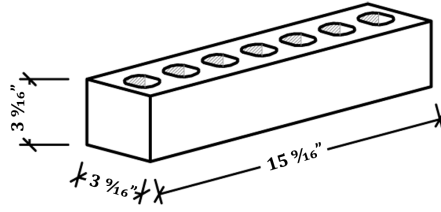
SUMMIT PLANT SUPER FOUR INCH (4x4x16)
