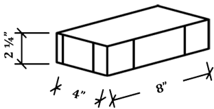
SUMMIT PLANT 4 x 8 LUGGED PAVER
