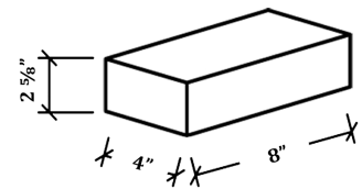
SUMMIT PLANT 4 x 8 HEAVY VEHICULAR PAVER
