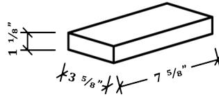
SUMMIT PLANT SPLIT MODULAR PAVER
